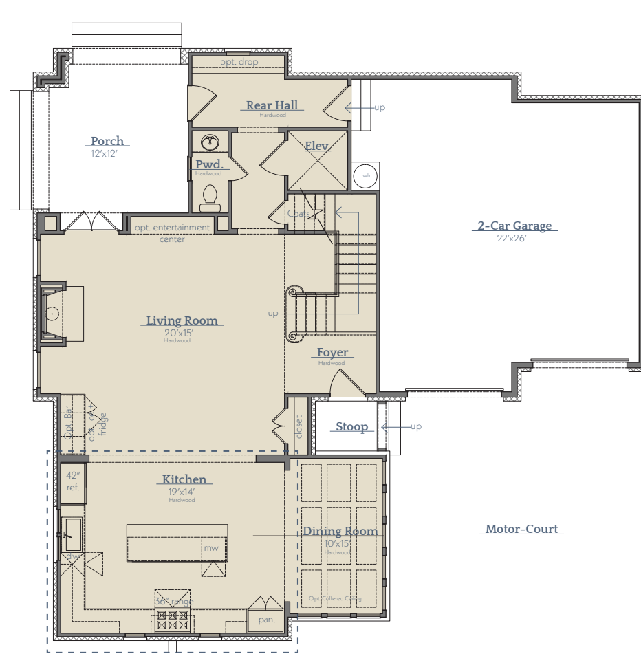
1st Floor
