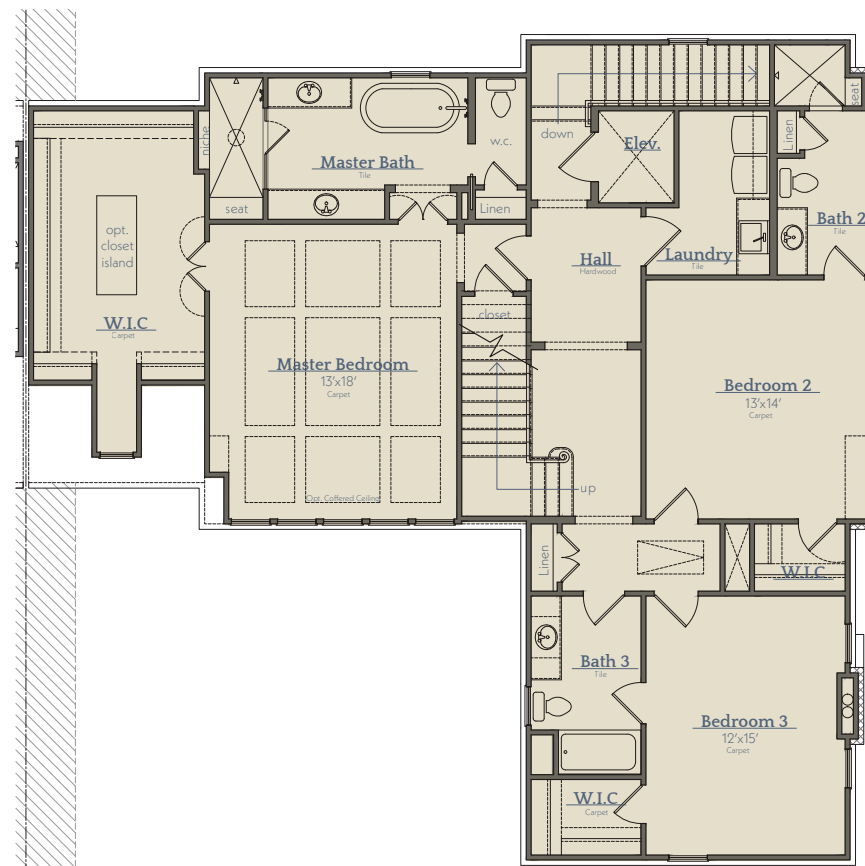
2nd Floor
